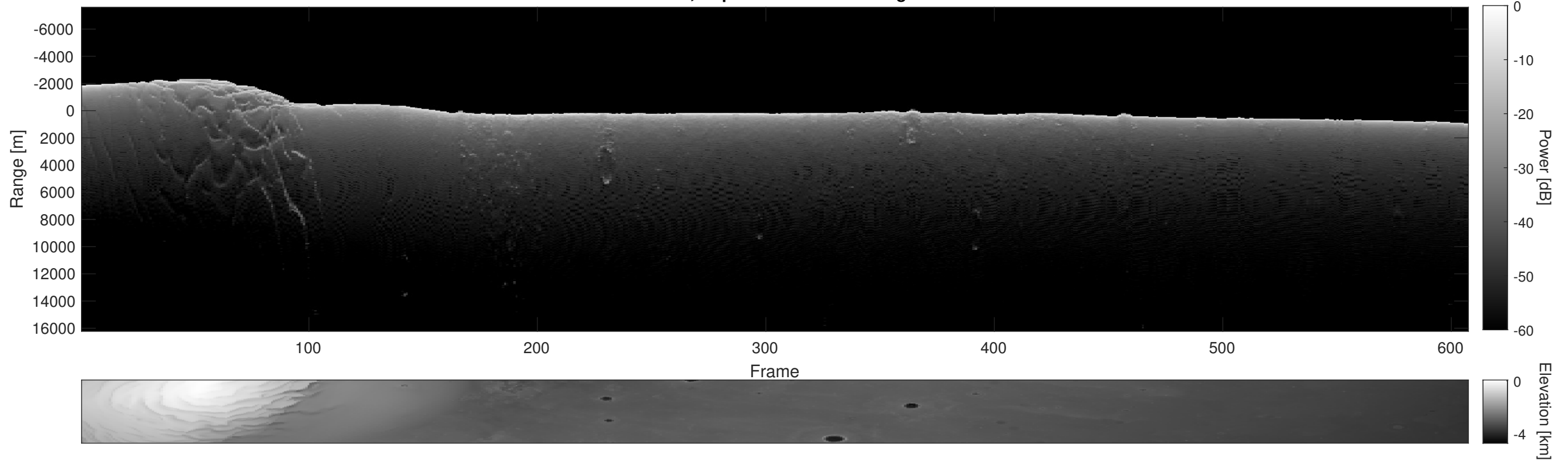
Orbit 7420, Depth-Corrected Cluttergram
