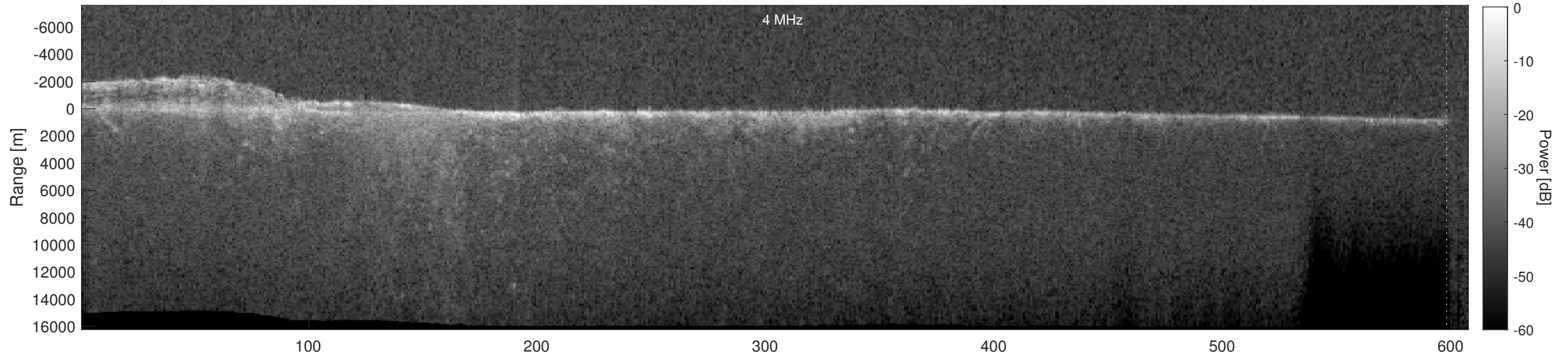
Orbit 7420, Depth-Corrected Cluttergram
