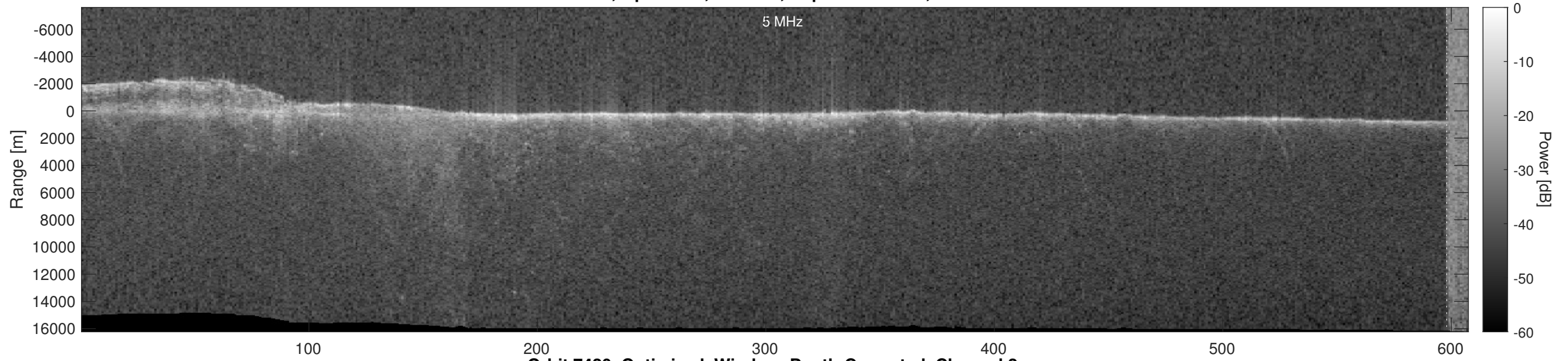
Orbit 7420, Optimized, Window, Depth-Corrected, Channel 2
