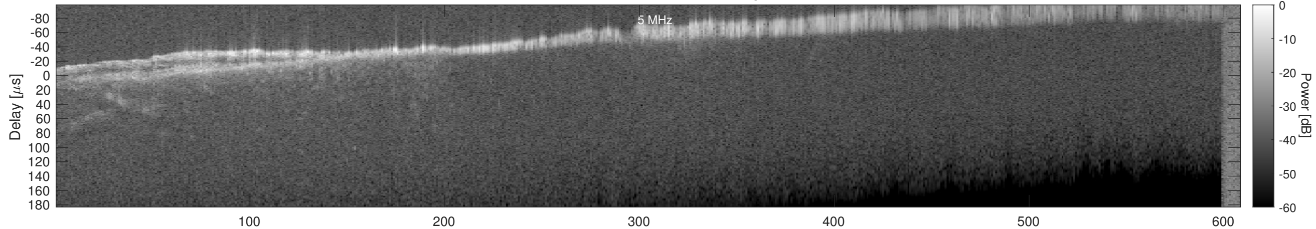
Orbit 7421, Window, Channel 1, Optimized
