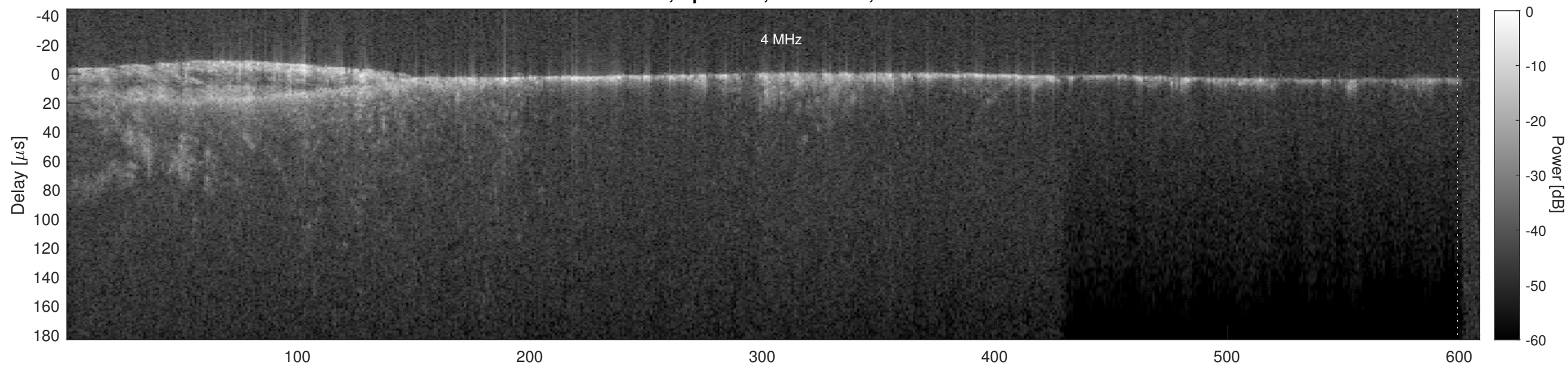
Orbit 7421, Cluttergram
