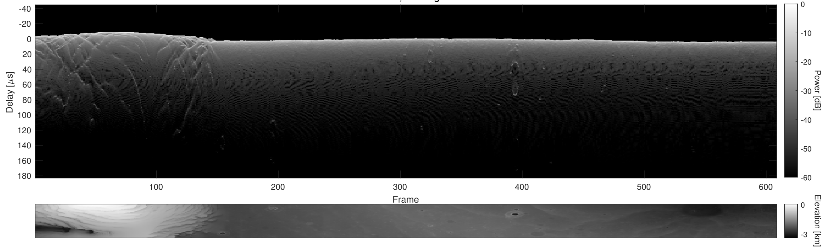
Orbit 7421, Cluttergram
