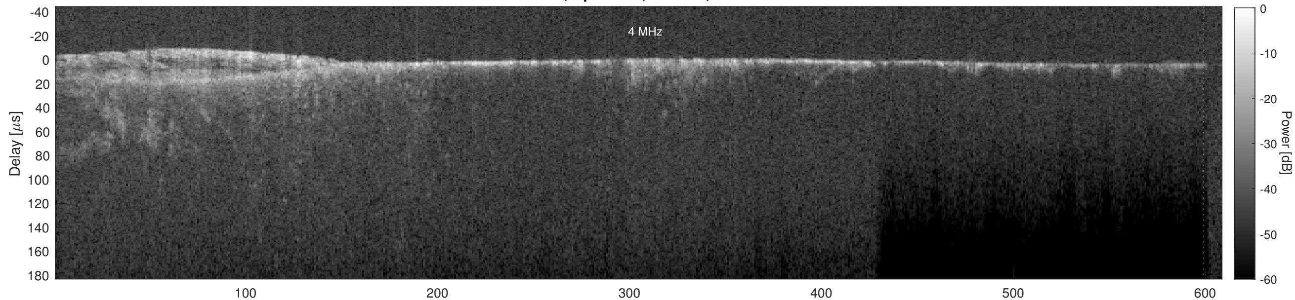
Orbit 7421, Cluttergram
