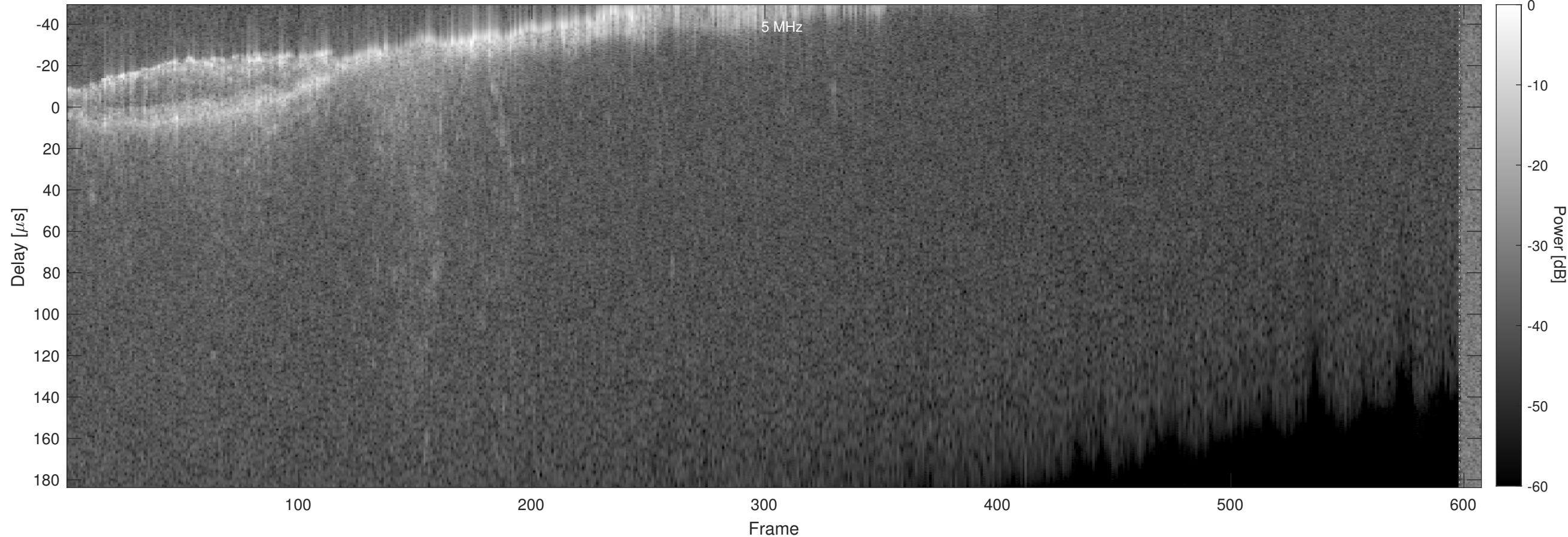
Orbit 7424, Chapman, No Window, Channel 2
