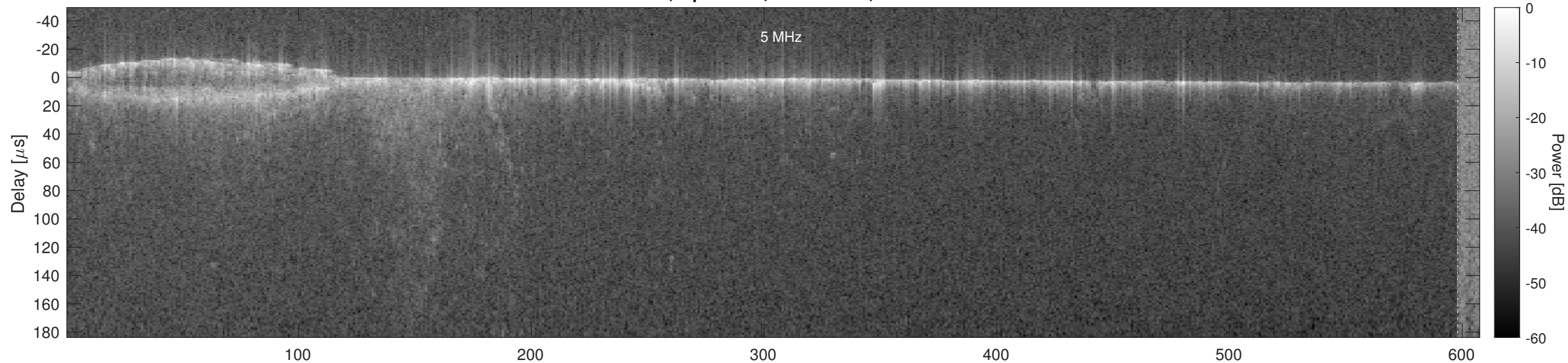
Orbit 7424, Optimized, No Window, Channel 2
