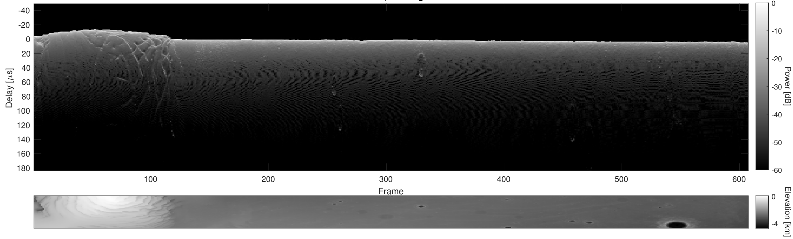
Orbit 7424, Cluttergram
