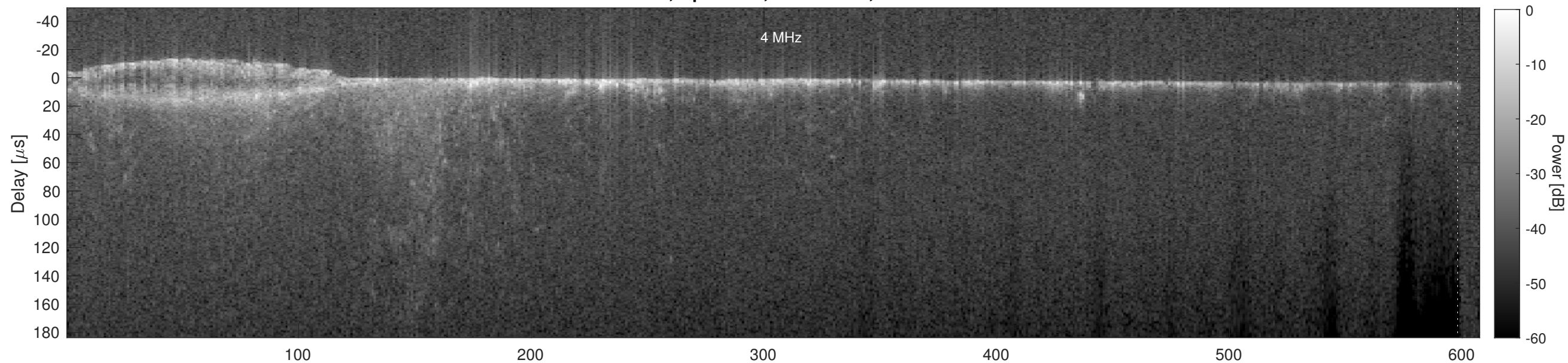
Orbit 7424, Cluttergram
