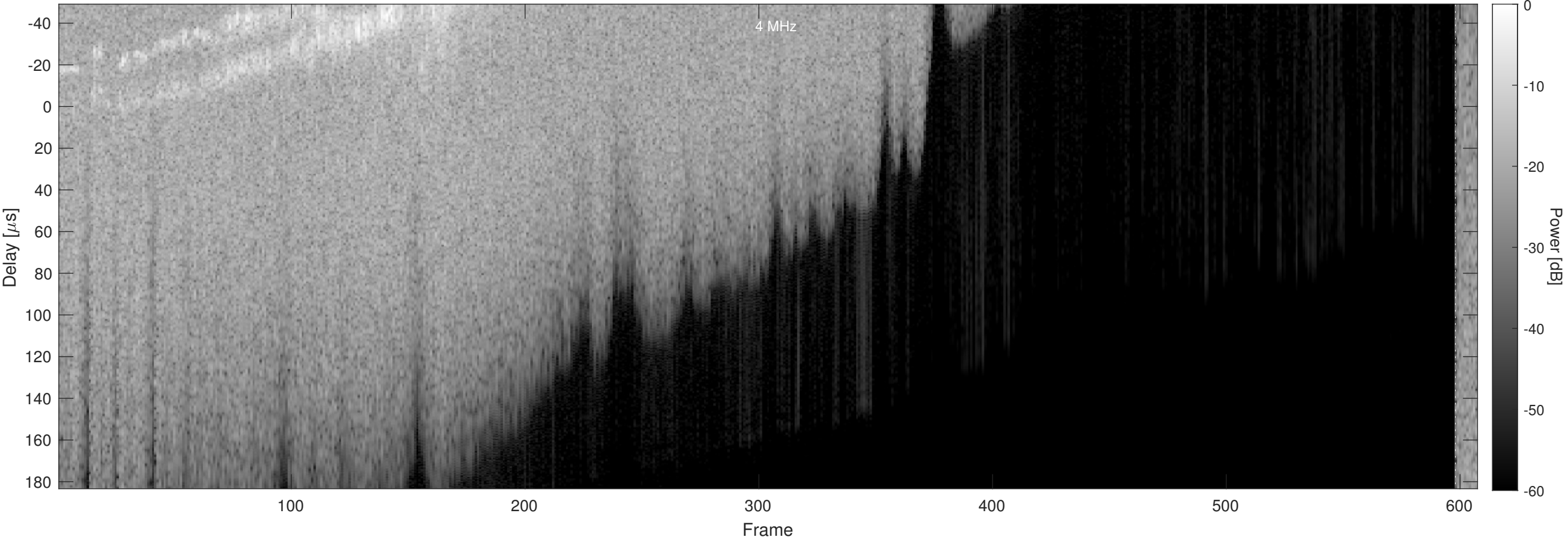
Orbit 7431, Chapman, Window, Channel 2
