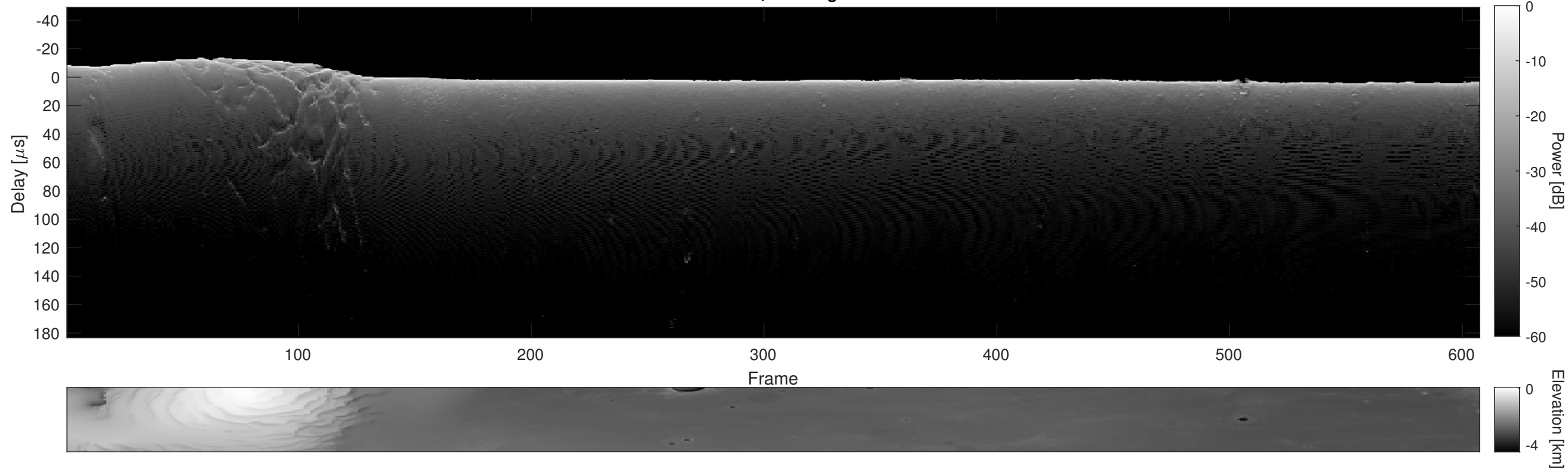
Orbit 7431, Cluttergram
