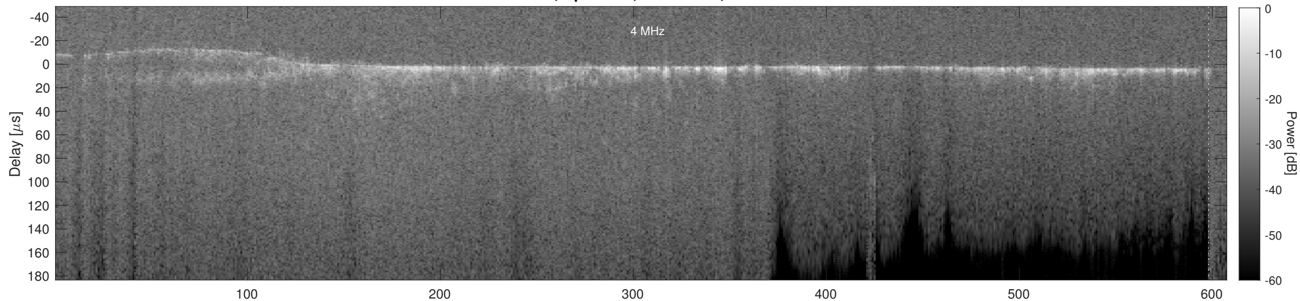
Orbit 7431, Cluttergram
