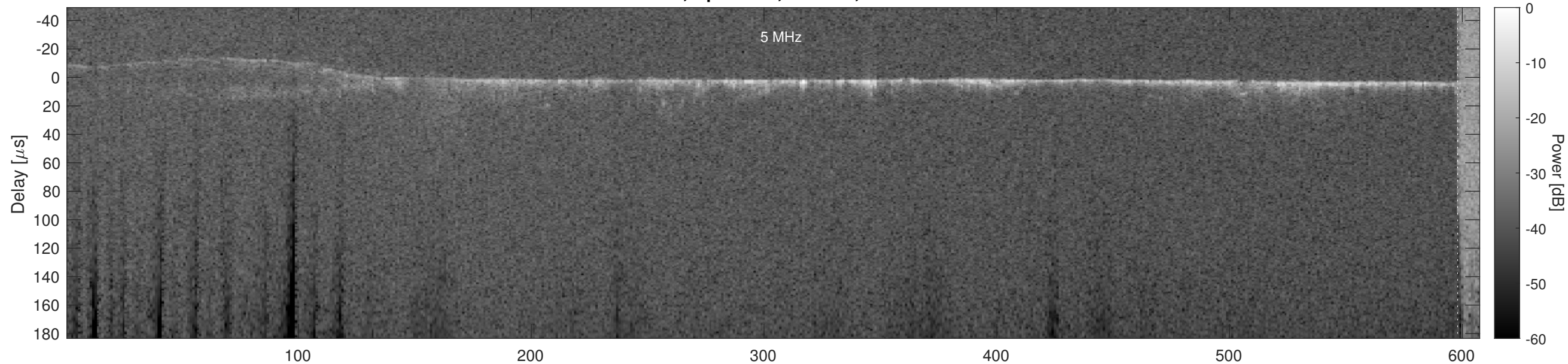
Orbit 7431, Optimized, Window, Channel 2
