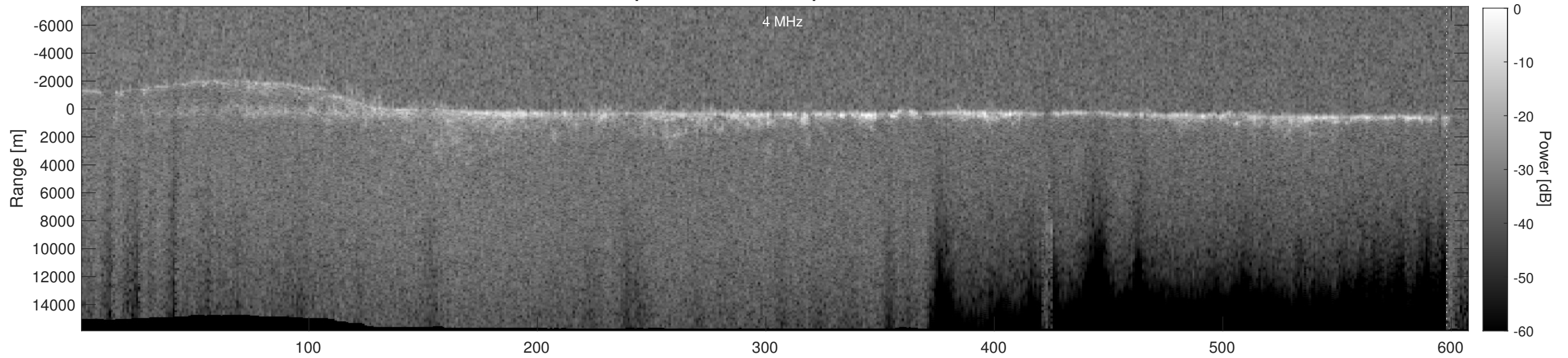
Orbit 7431, Depth-Corrected Cluttergram
