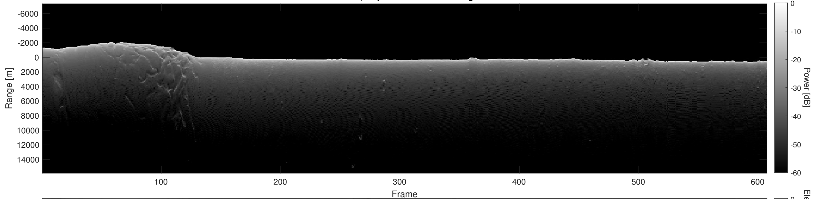
Orbit 7431, Depth-Corrected Cluttergram
