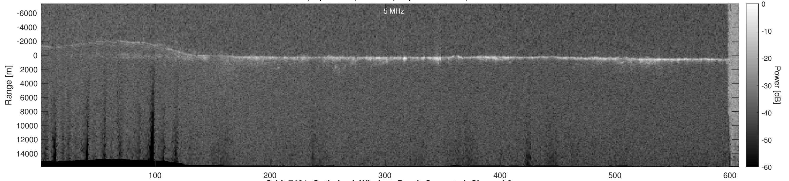
Orbit 7431, Optimized, Window, Depth-Corrected, Channel 2
