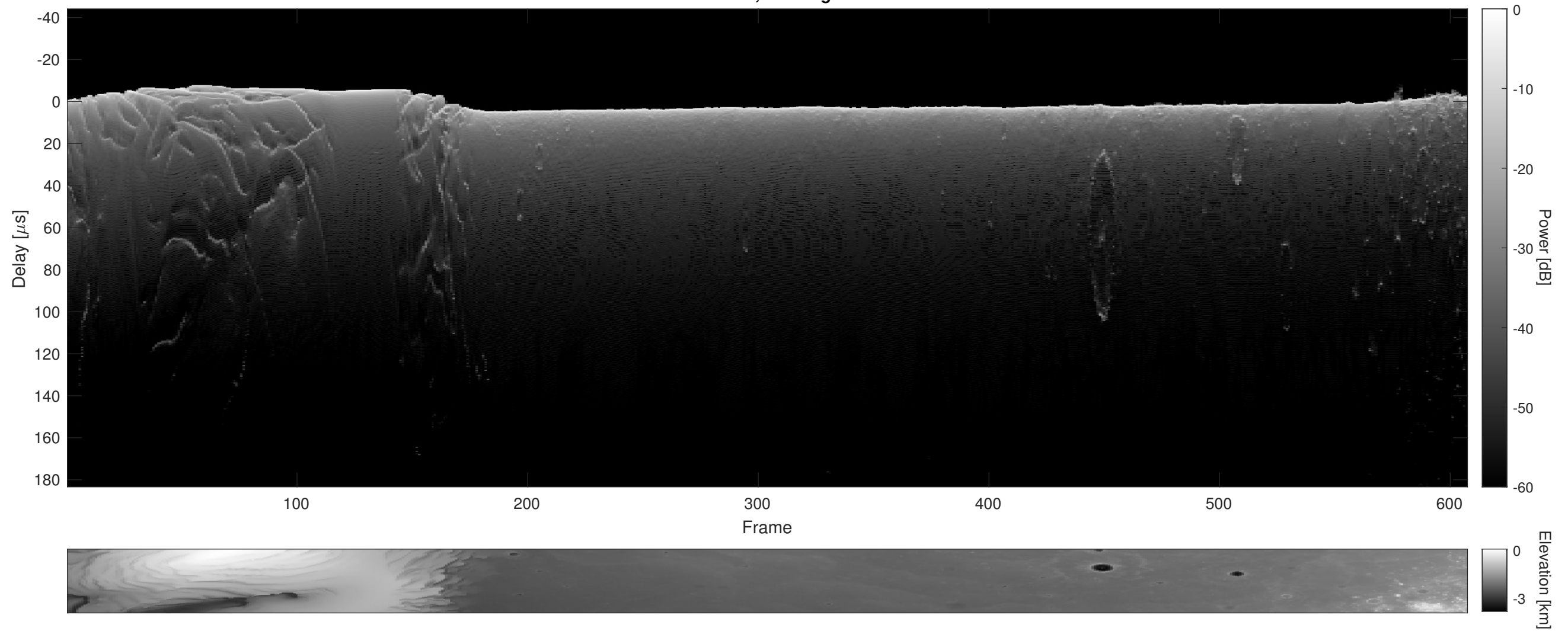
Orbit 7432, Cluttergram
