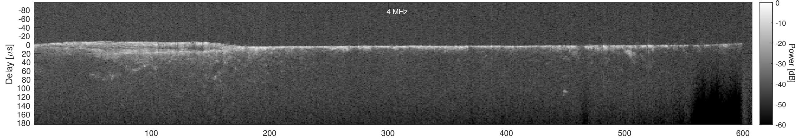
Orbit 7432, Cluttergram
