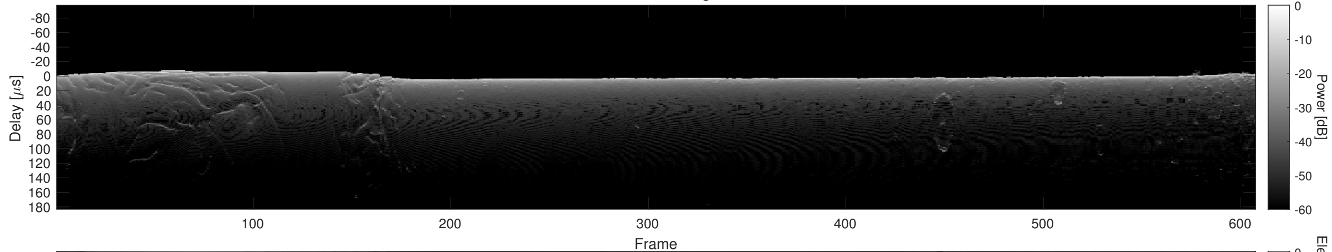
Orbit 7432, Cluttergram
