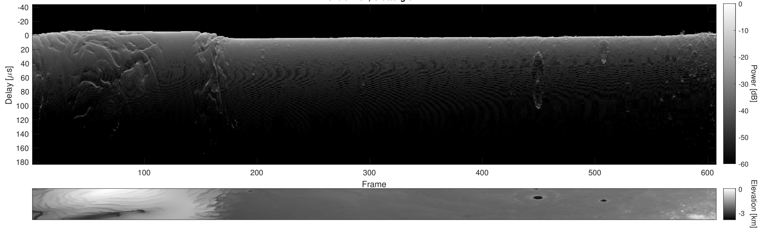
Orbit 7432, Cluttergram
