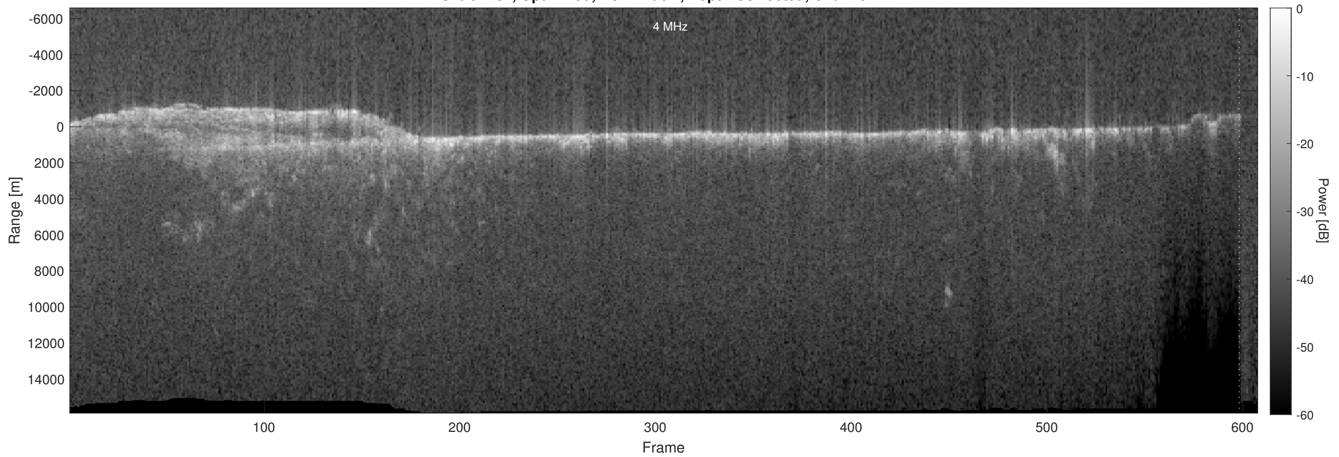
Orbit 7432, Optimized, No Window, Depth-Corrected, Channel 2
