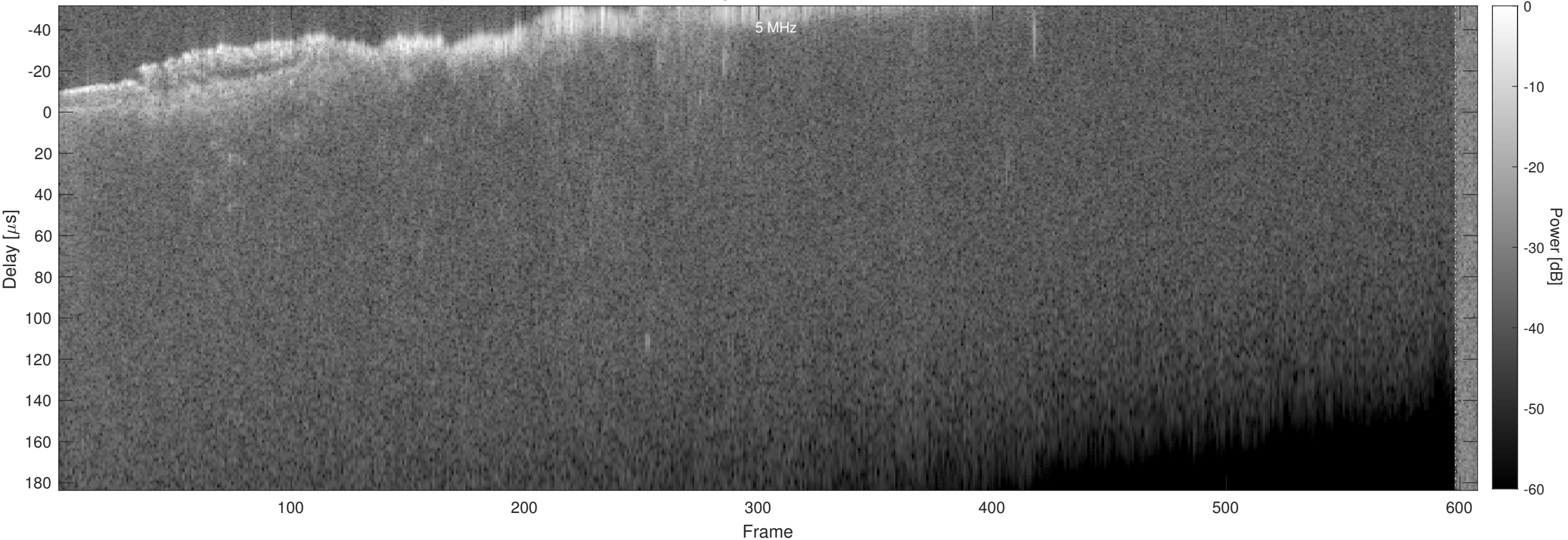
Orbit 7433, Chapman, Window, Channel 2
