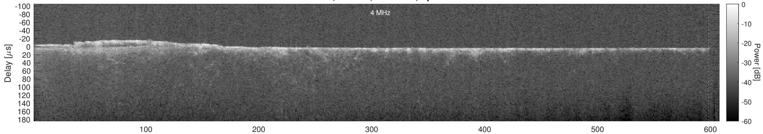
Orbit 7433, Cluttergram
