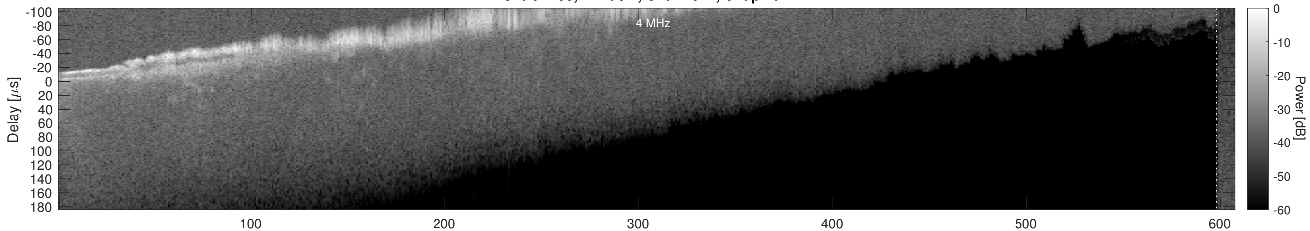
Orbit 7433, Window, Channel 2, Optimized
