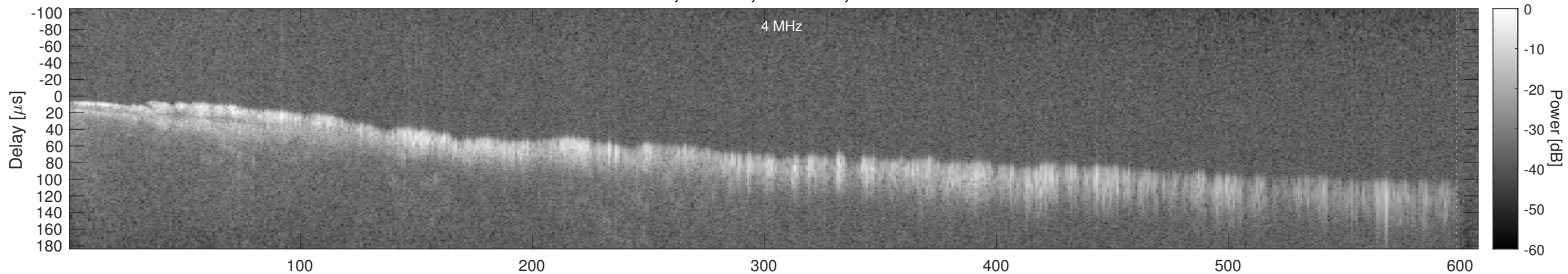
Orbit 7433, Window, Channel 2, Chapman
