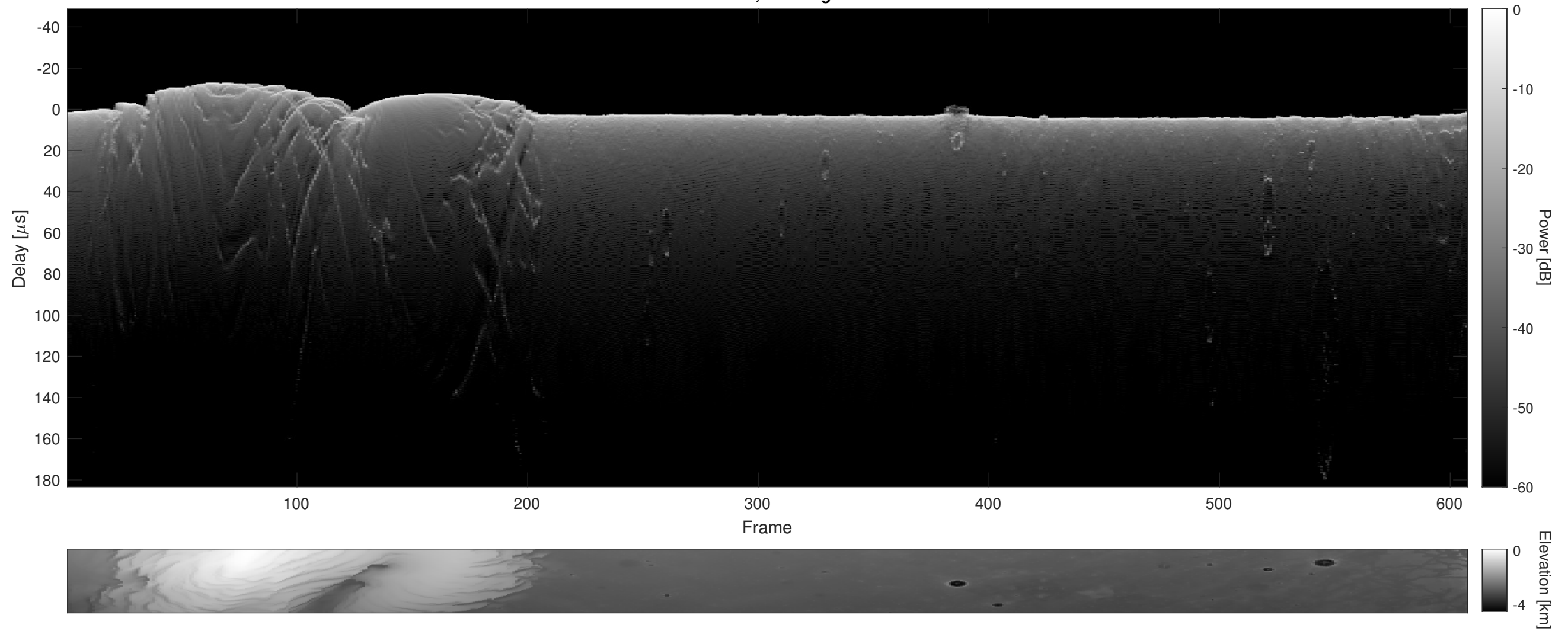
Orbit 7436, Cluttergram
