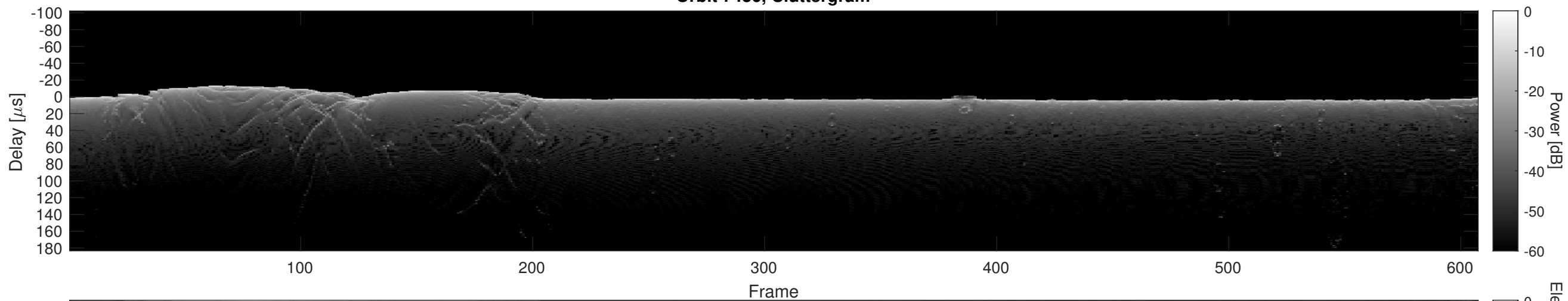
Orbit 7436, Cluttergram
