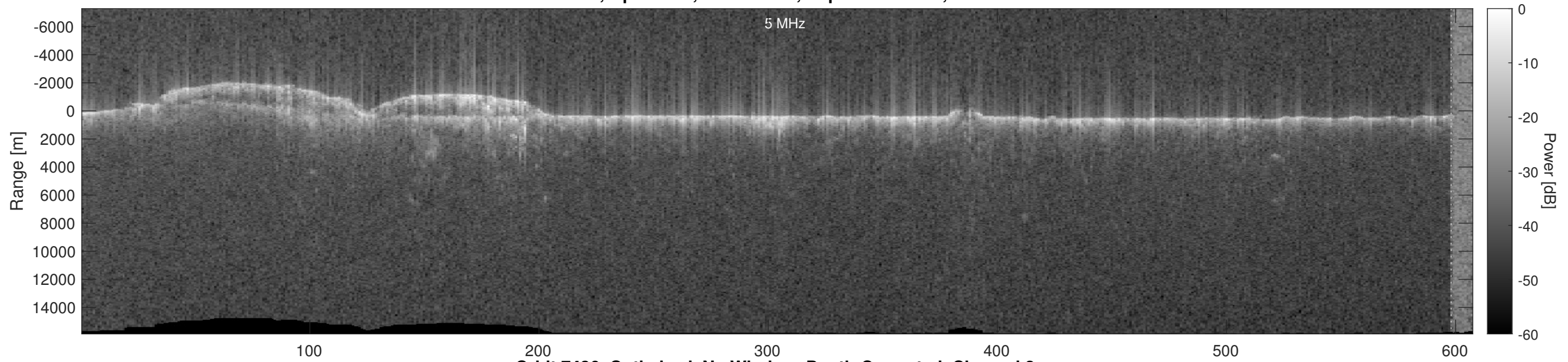
Orbit 7436, Optimized, No Window, Depth-Corrected, Channel 2
