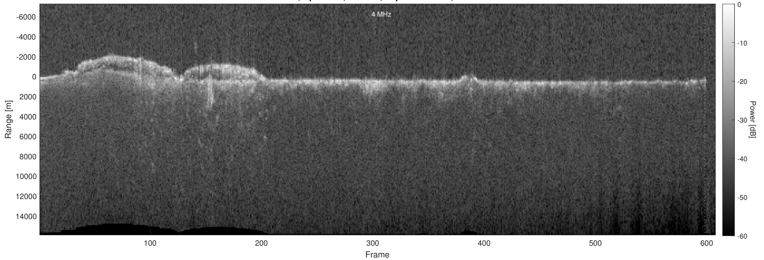
Orbit 7436, Optimized, Window, Depth-Corrected, Channel 2
