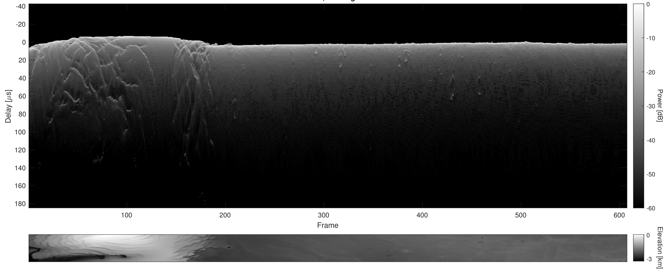
Orbit 7439, Cluttergram
