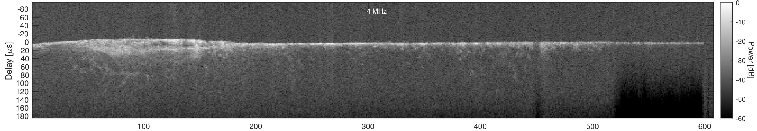
Orbit 7439, Cluttergram
