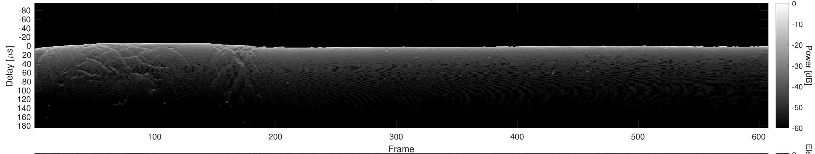
Orbit 7439, Cluttergram
