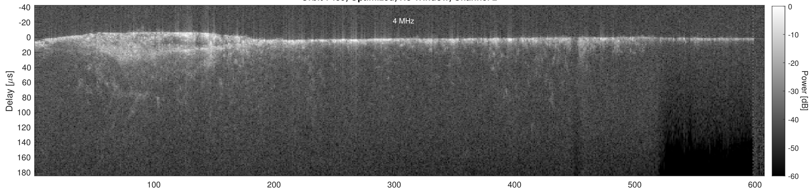
Orbit 7439, Cluttergram
