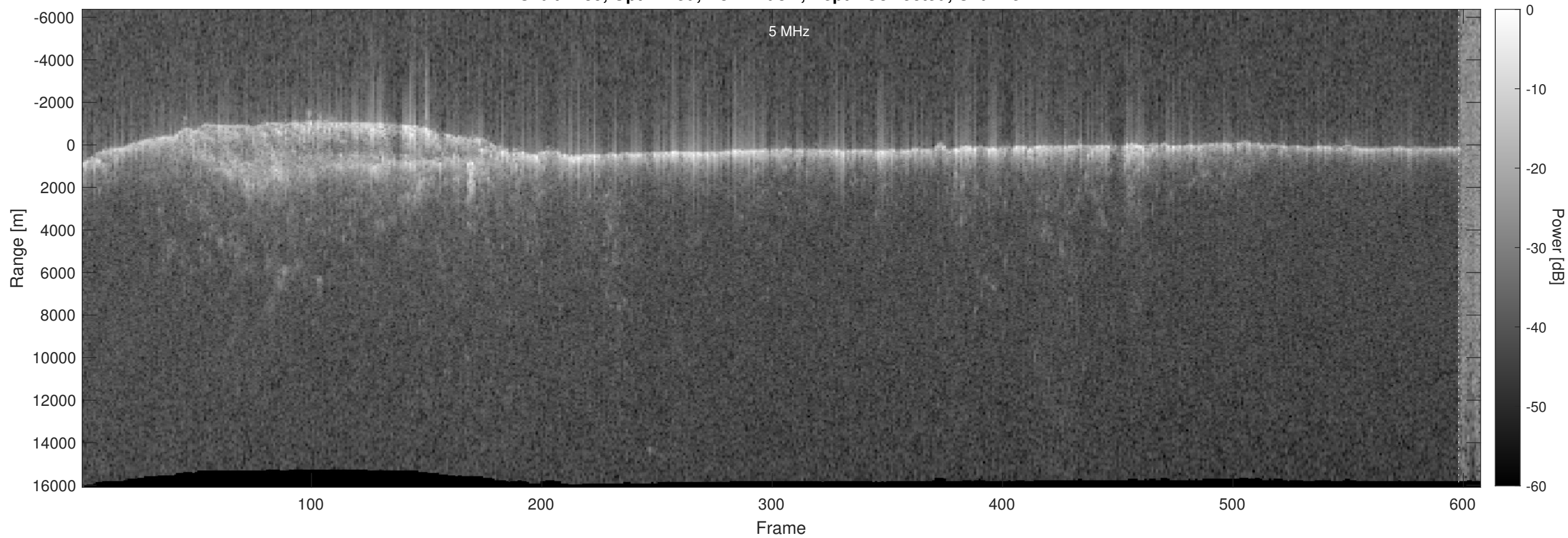
Orbit 7439, Optimized, No Window, Depth-Corrected, Channel 2
