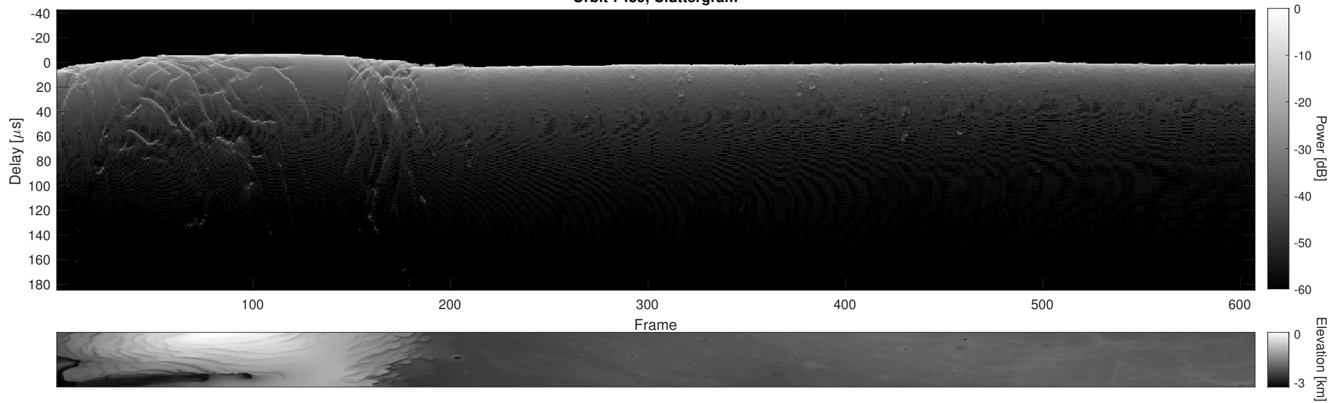
Orbit 7439, Cluttergram
