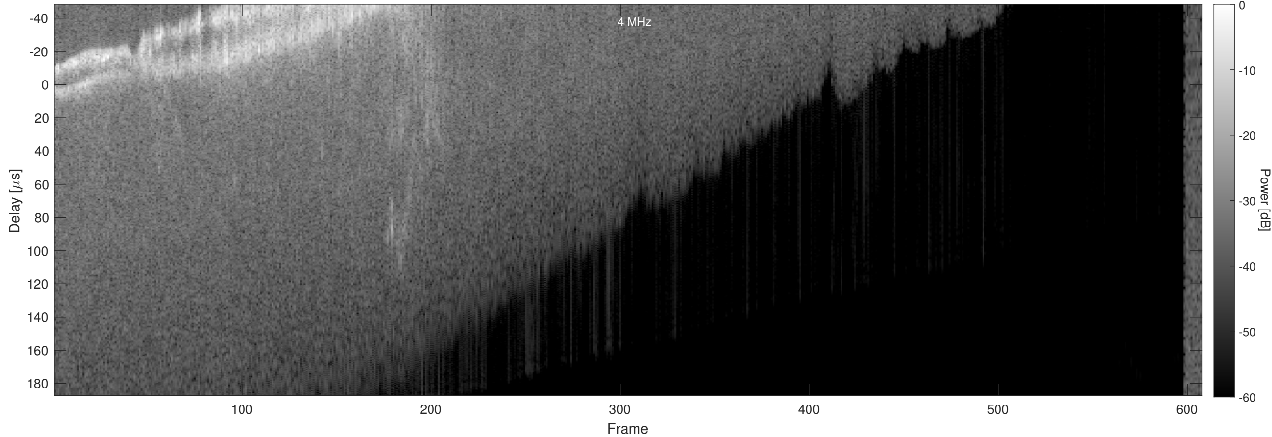
Orbit 7442, Chapman, No Window, Channel 2
