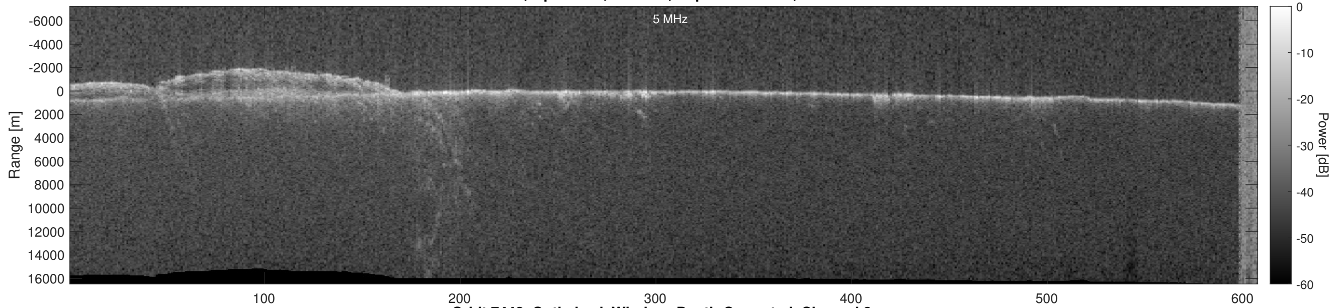
Orbit 7442, Optimized, Window, Depth-Corrected, Channel 2
