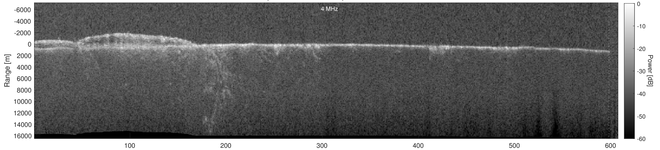
Orbit 7442, Depth-Corrected Cluttergram
