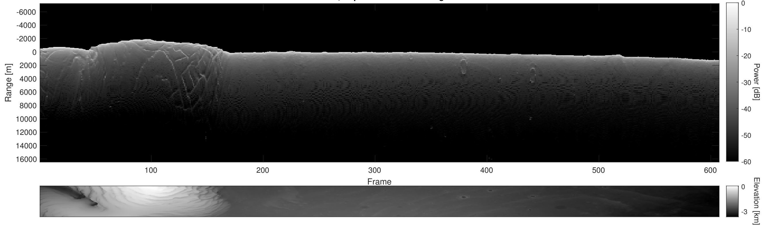
Orbit 7442, Depth-Corrected Cluttergram
