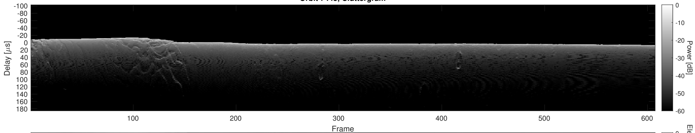
Orbit 7445, Cluttergram
