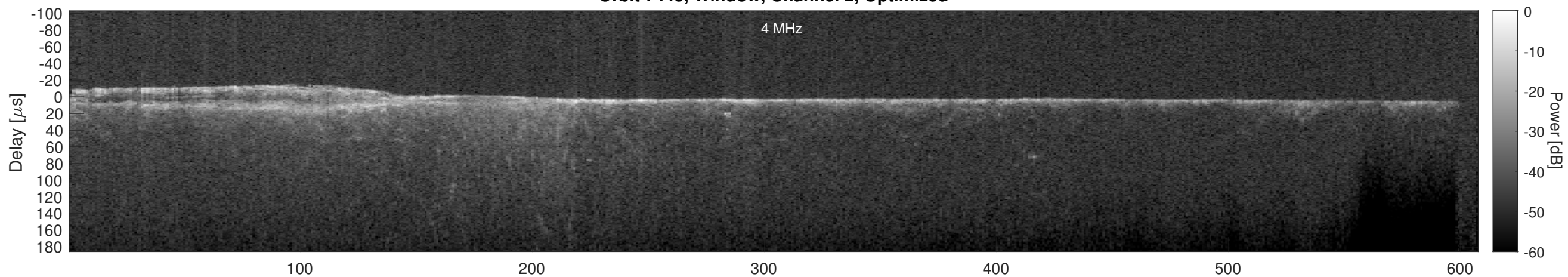
Orbit 7445, Cluttergram
