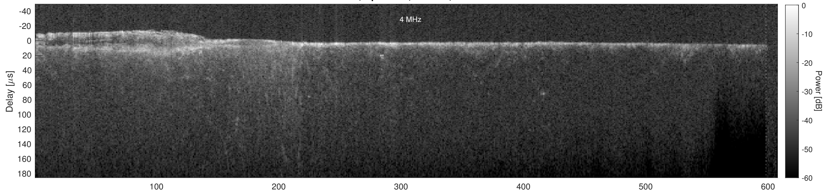
Orbit 7445, Cluttergram
