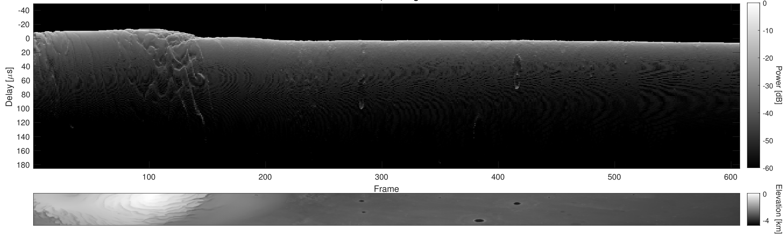
Orbit 7445, Cluttergram
