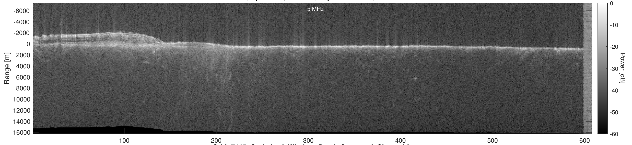
Orbit 7445, Optimized, Window, Depth-Corrected, Channel 2
