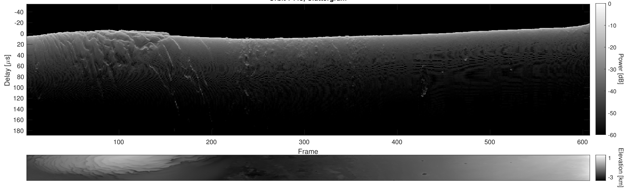
Orbit 7448, Cluttergram
