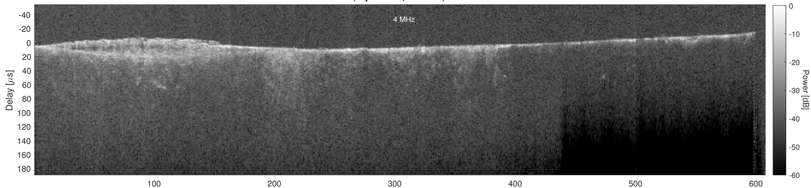
Orbit 7448, Cluttergram
