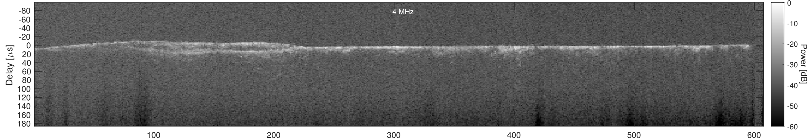
Orbit 7450, Cluttergram
