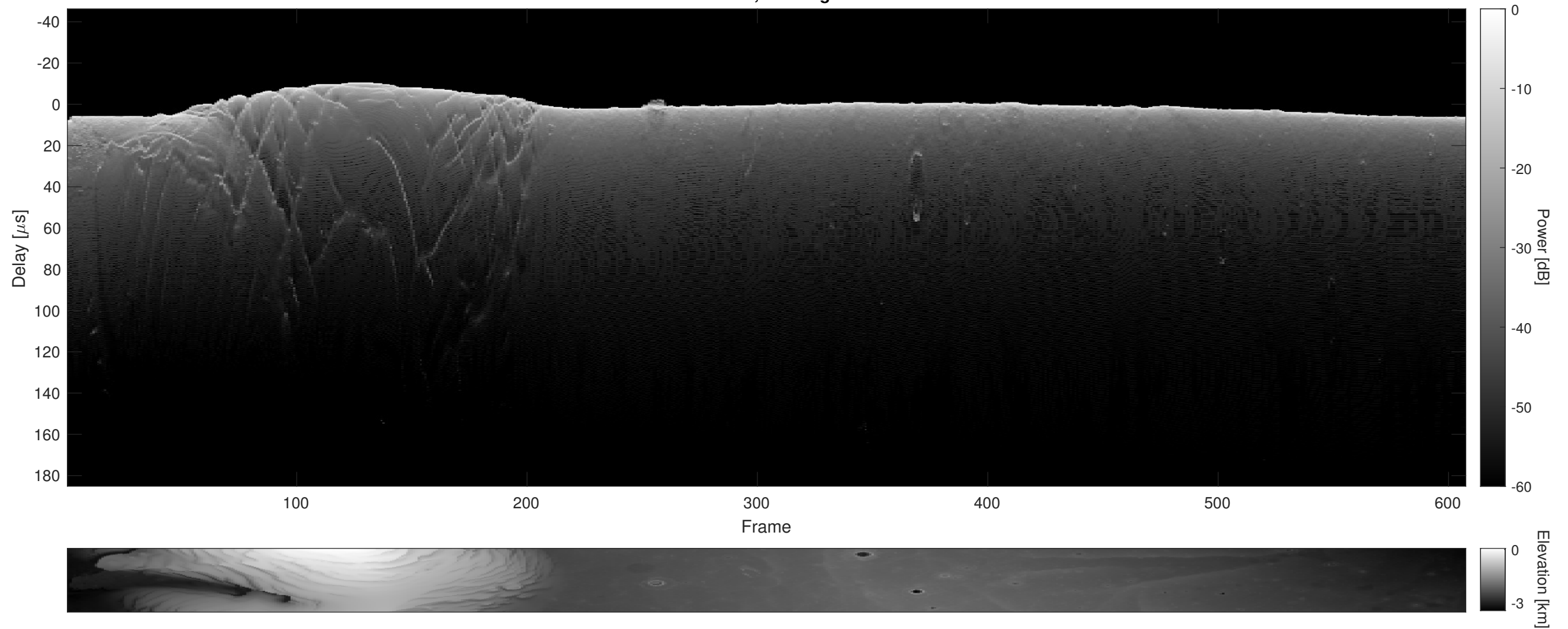
Orbit 7453, Cluttergram
