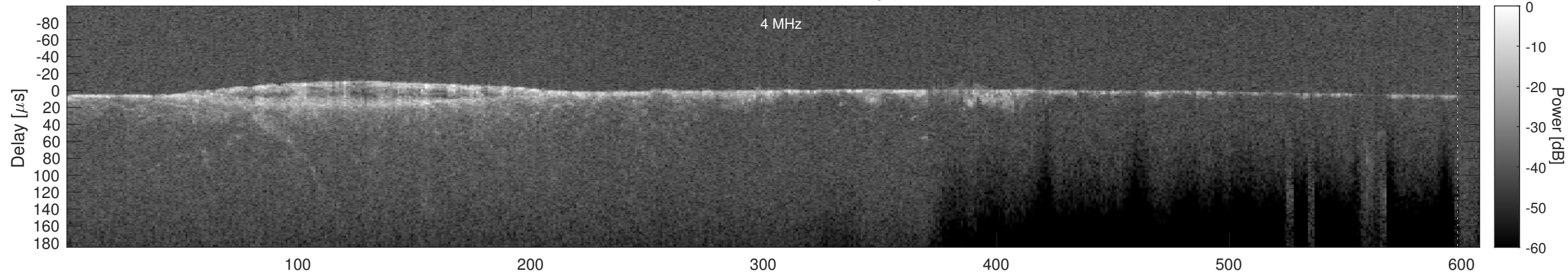
Orbit 7453, Cluttergram
