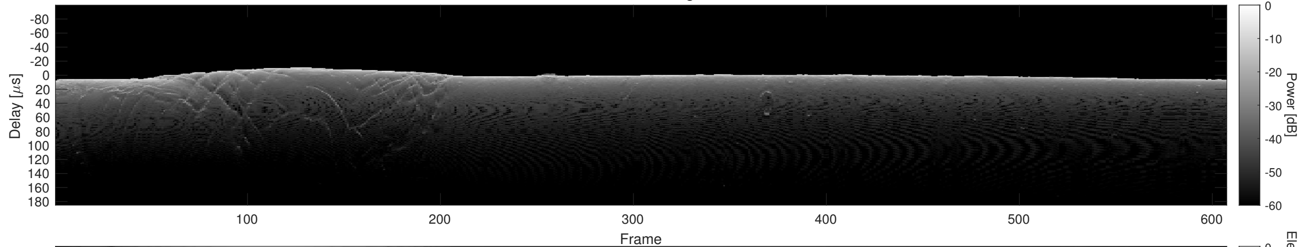
Orbit 7453, Cluttergram
