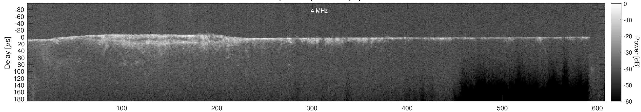
Orbit 7457, Cluttergram
