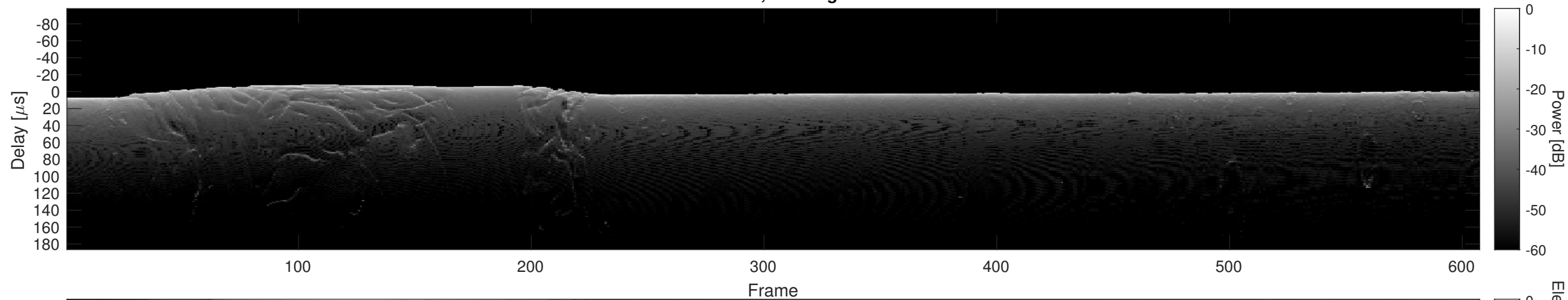
Orbit 7457, Cluttergram
