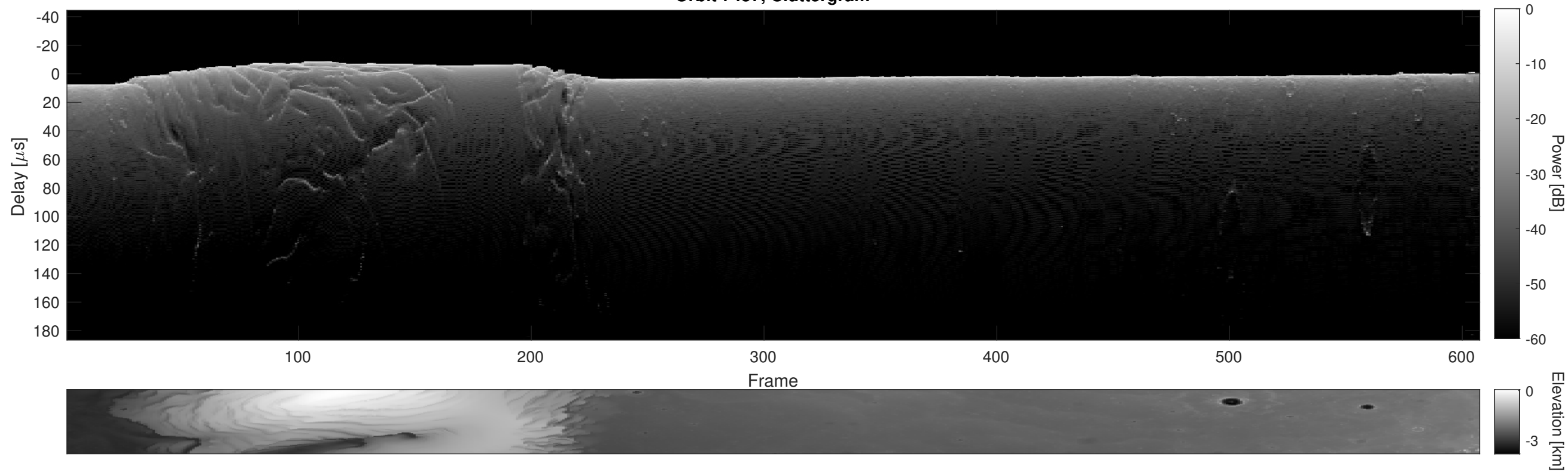
Orbit 7457, Cluttergram
