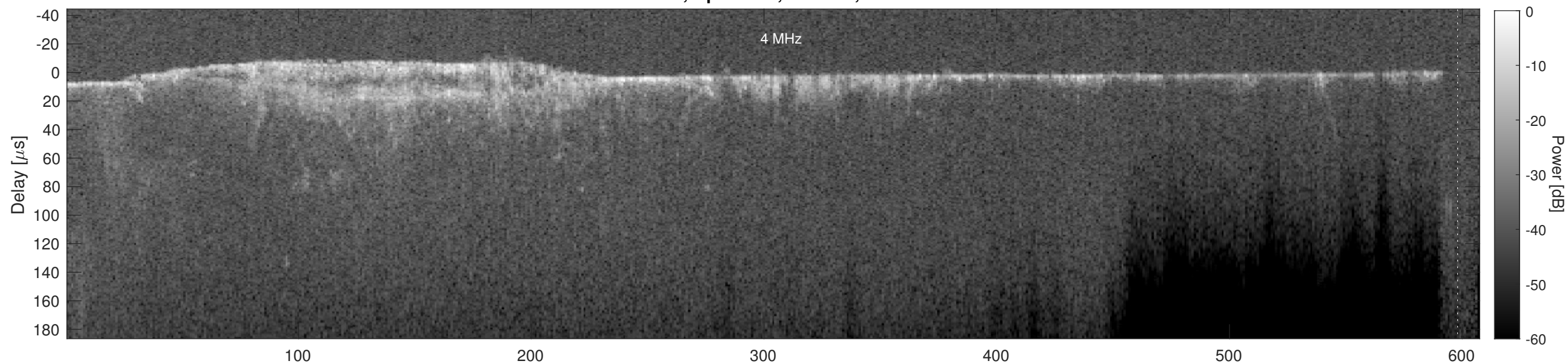
Orbit 7457, Cluttergram
