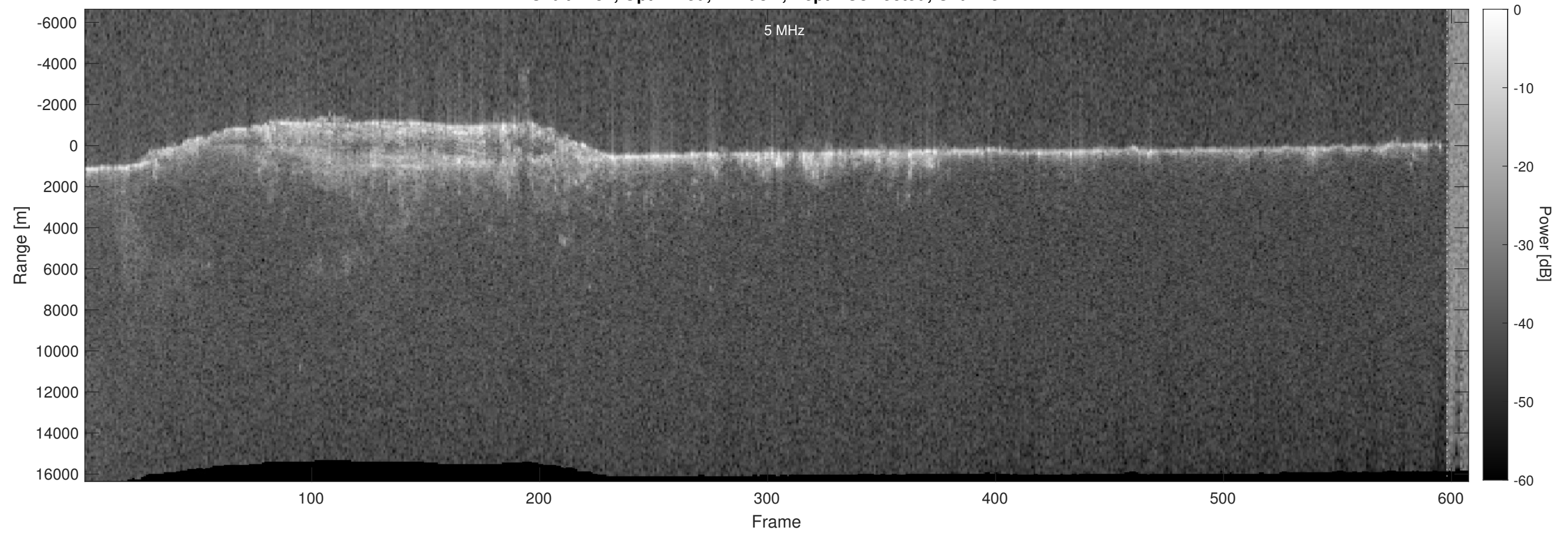
Orbit 7457, Optimized, Window, Depth-Corrected, Channel 2
