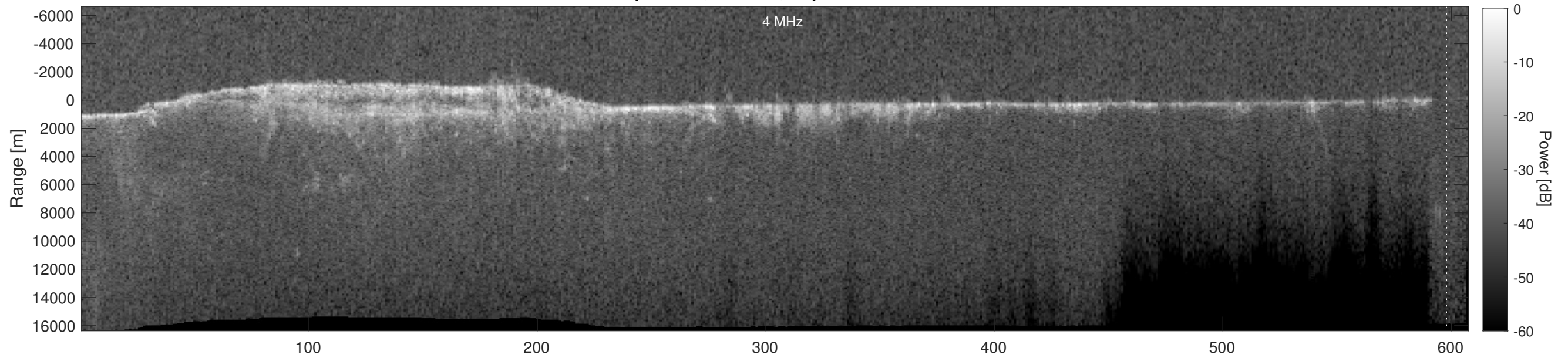
Orbit 7457, Depth-Corrected Cluttergram
