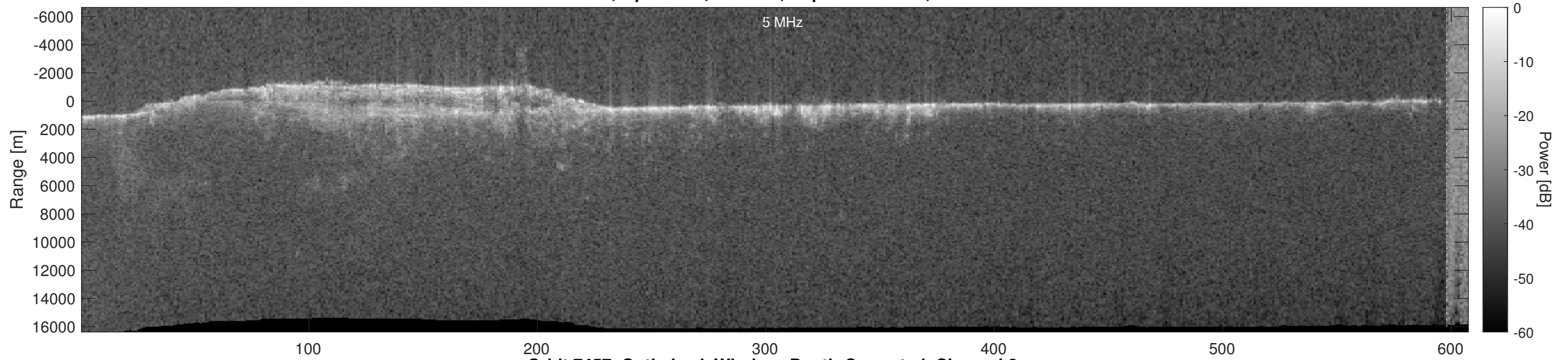
Orbit 7457, Optimized, Window, Depth-Corrected, Channel 2
