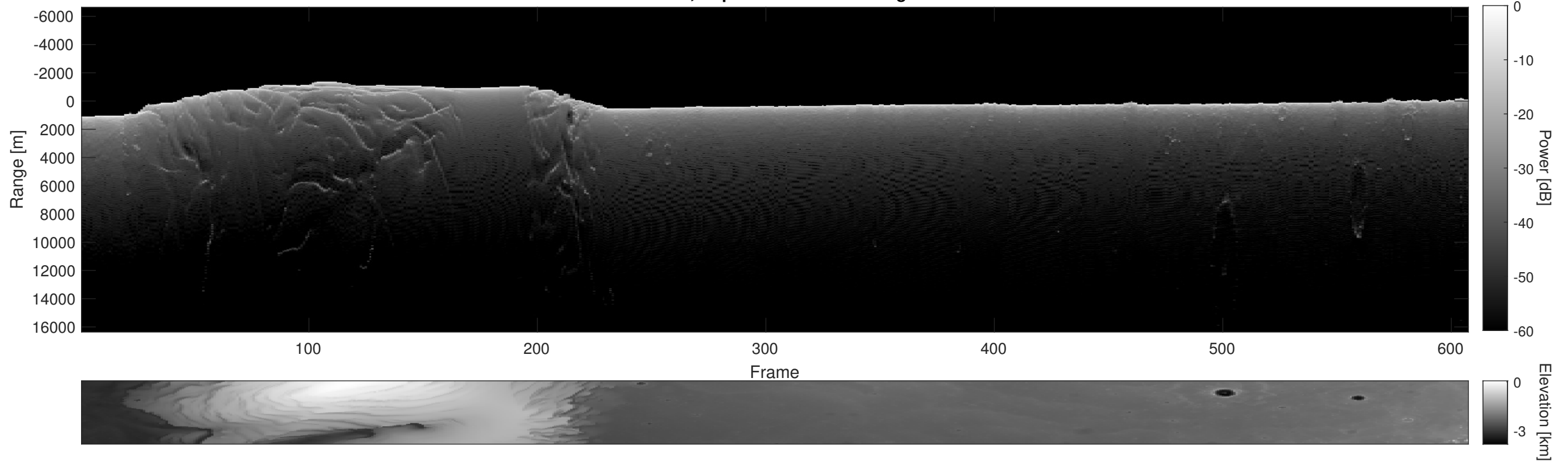
Orbit 7457, Depth-Corrected Cluttergram
