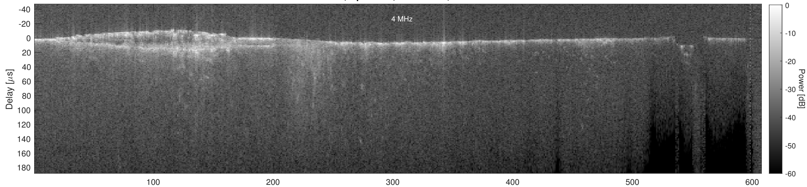
Orbit 7459, Cluttergram
