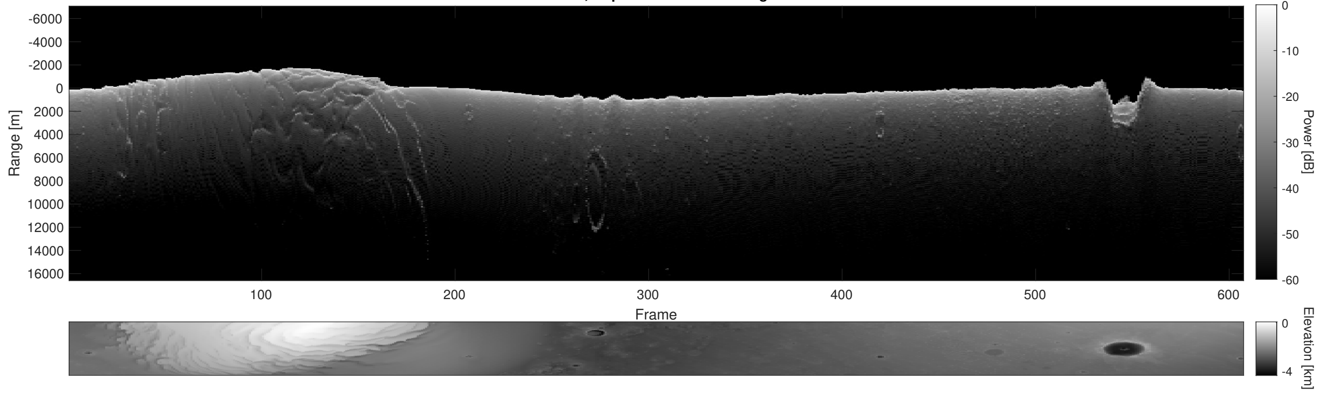
Orbit 7459, Depth-Corrected Cluttergram
