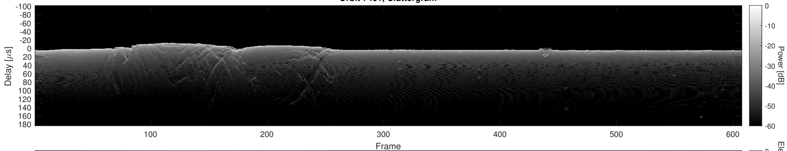
Orbit 7461, Cluttergram
