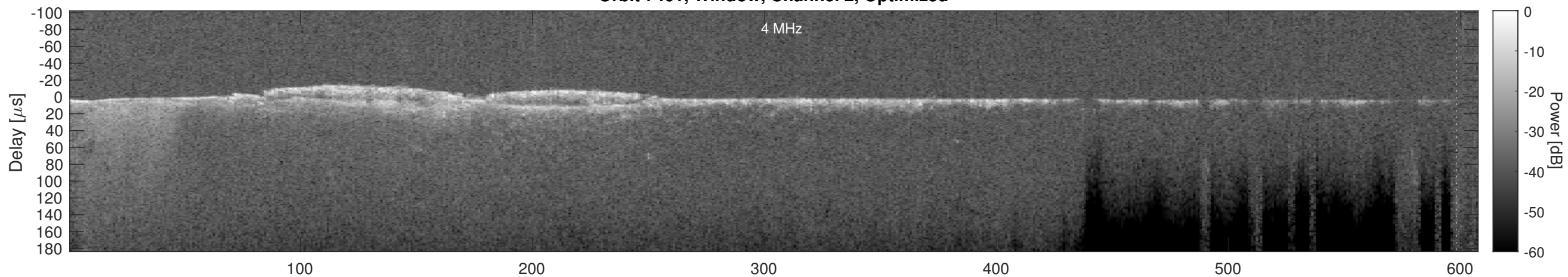
Orbit 7461, Cluttergram
