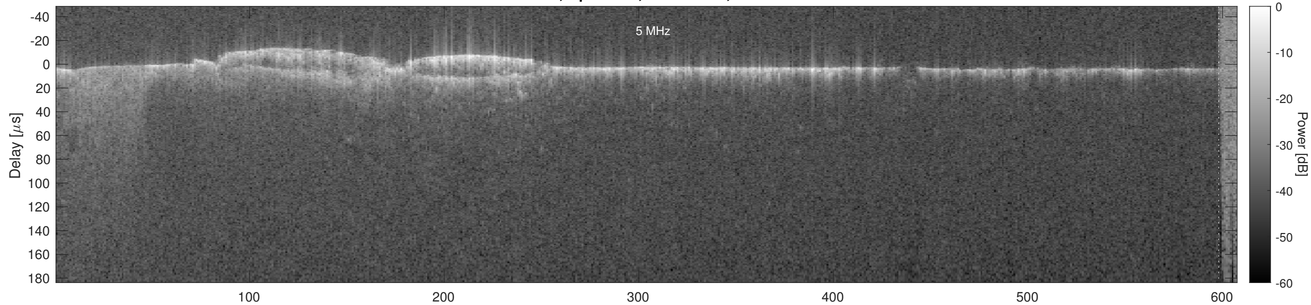
Orbit 7461, Optimized, No Window, Channel 2
