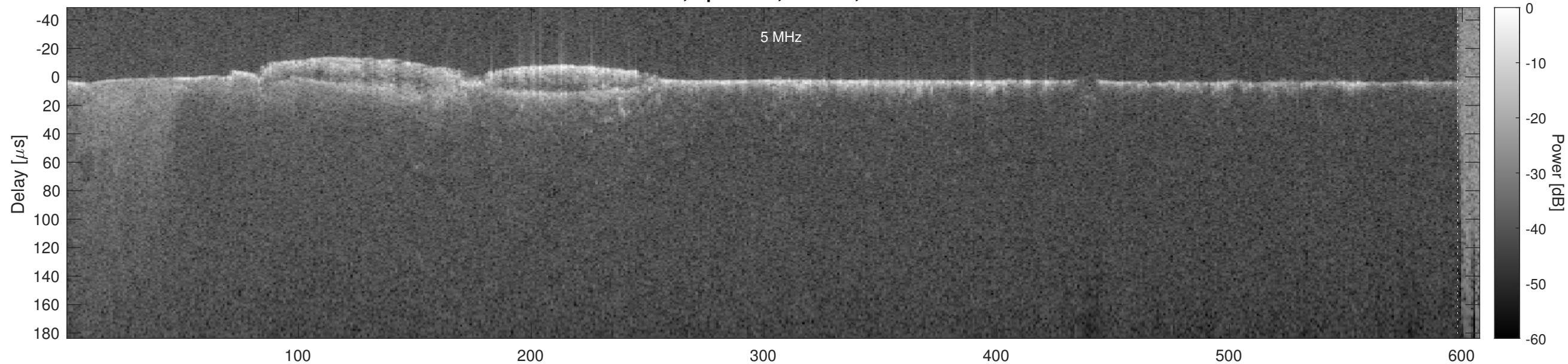
Orbit 7461, Optimized, Window, Channel 2
