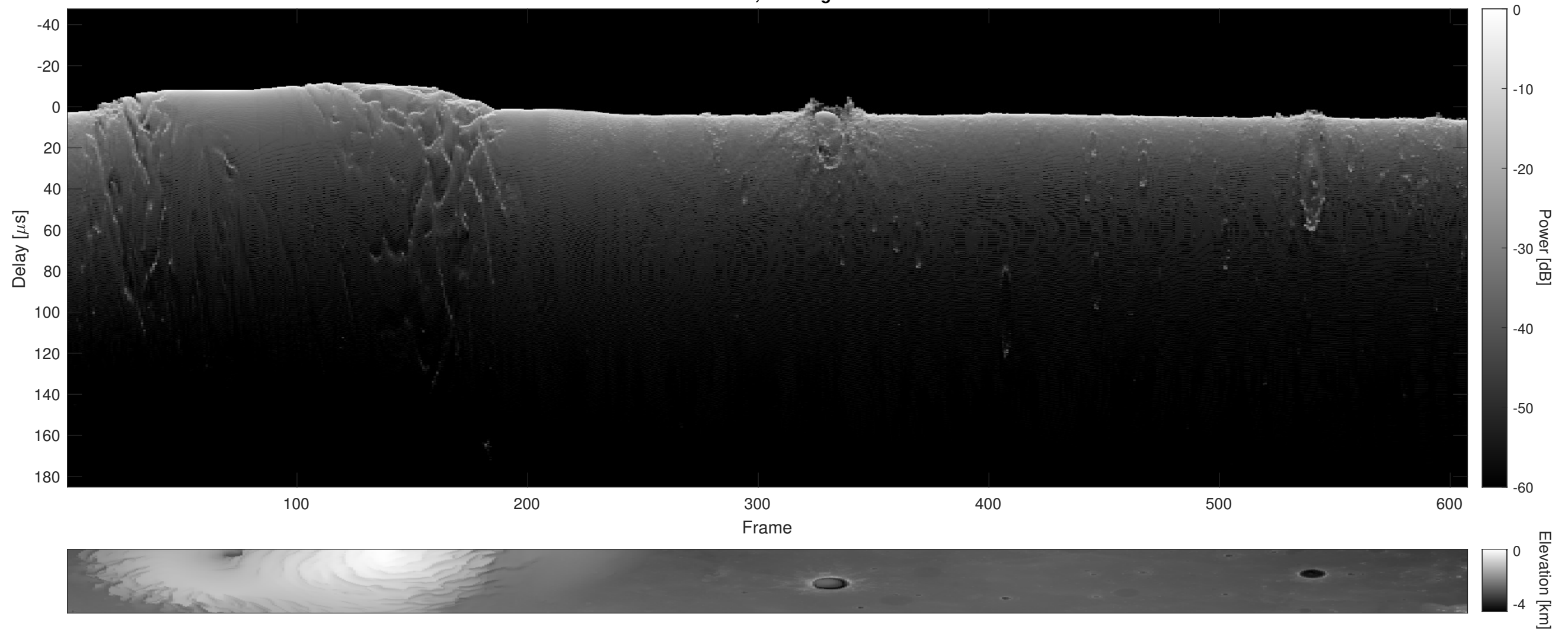
Orbit 7463, Cluttergram
