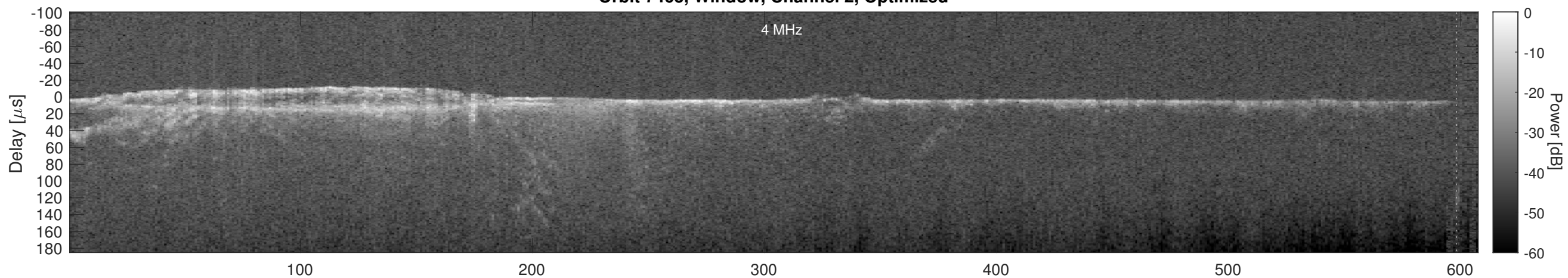
Orbit 7463, Cluttergram
