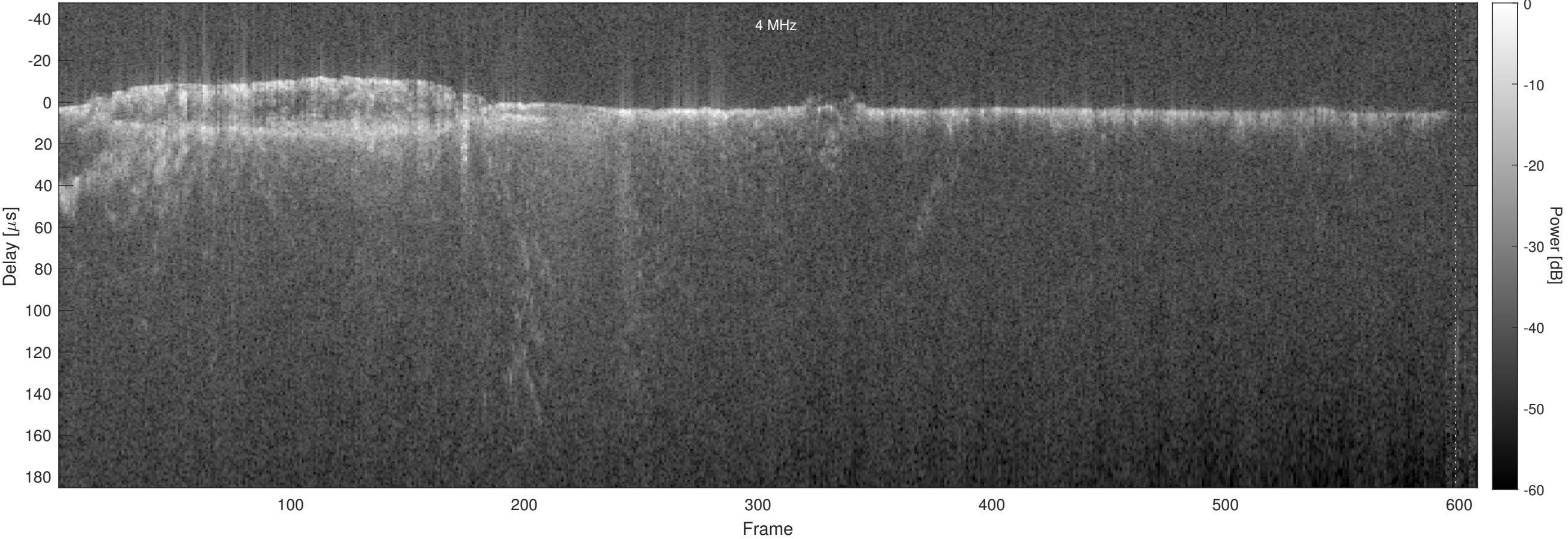
Orbit 7463, Optimized, No Window, Channel 2
