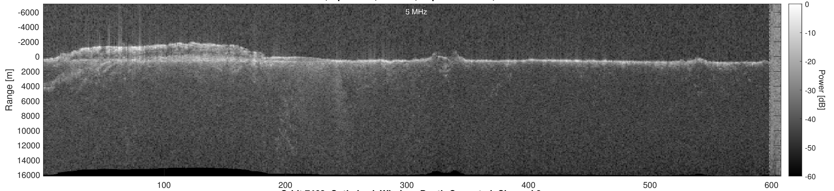
Orbit 7463, Optimized, Window, Depth-Corrected, Channel 2
