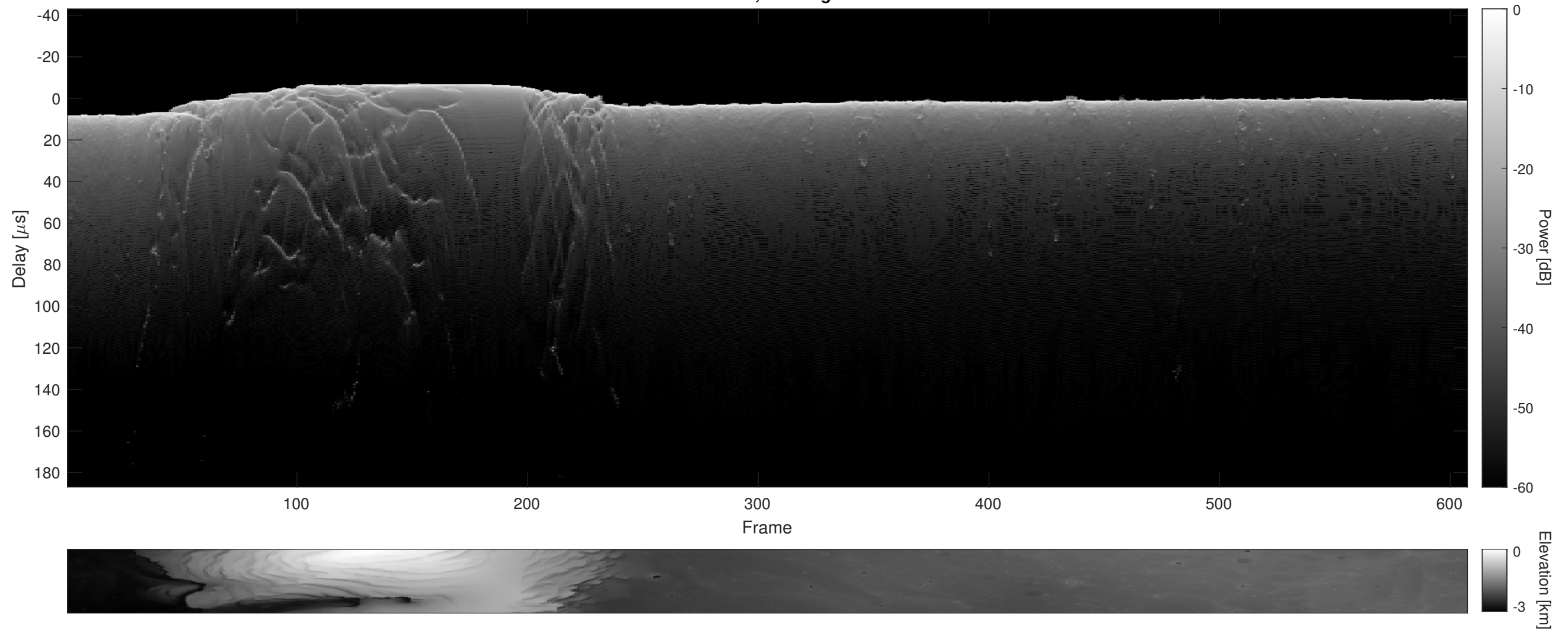
Orbit 7464, Cluttergram
