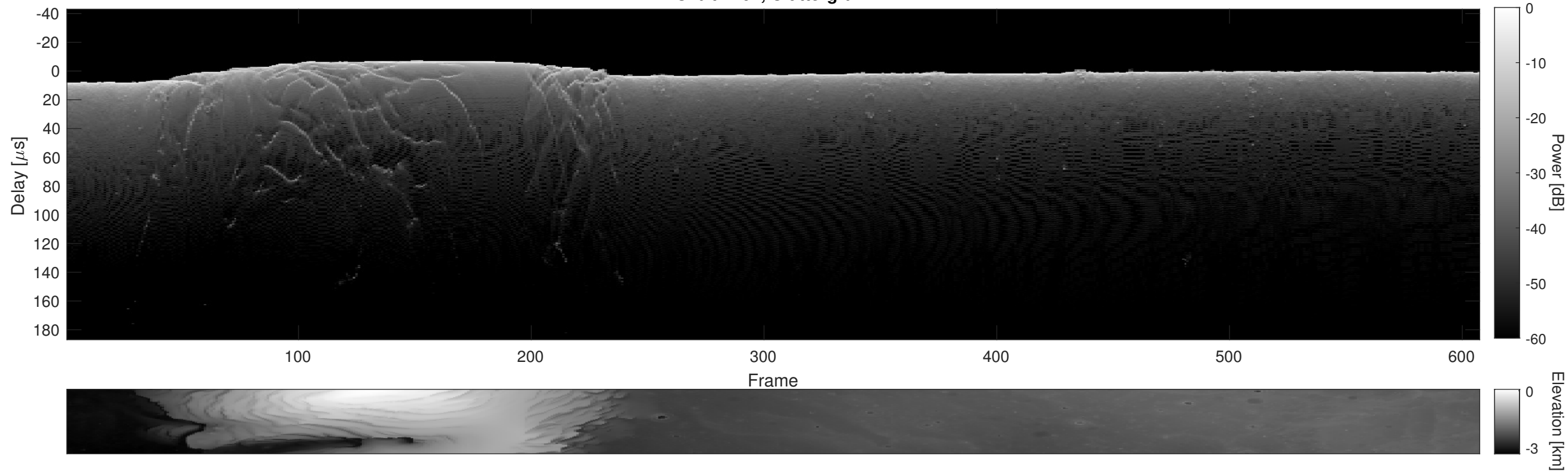
Orbit 7464, Cluttergram
