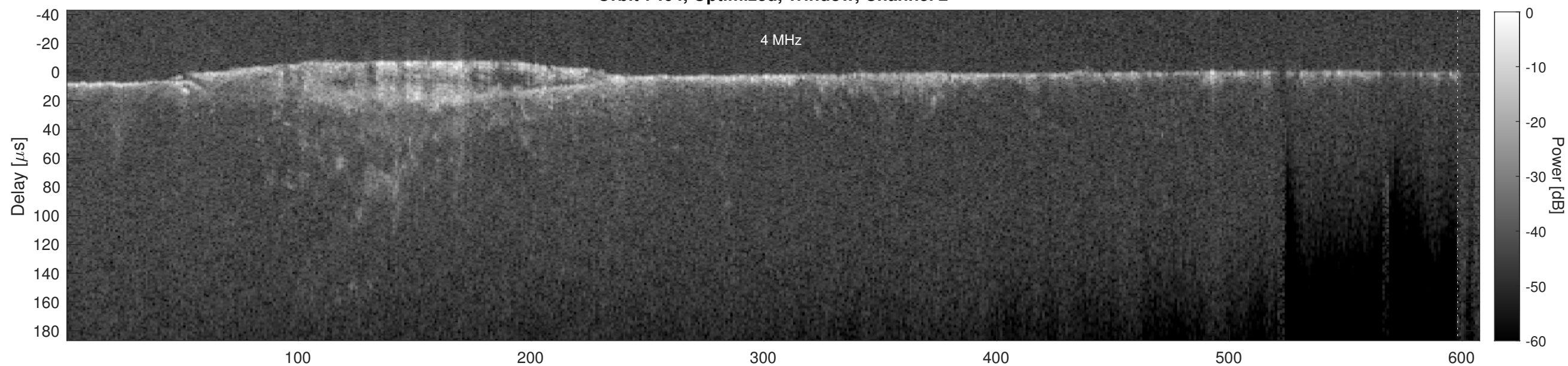
Orbit 7464, Cluttergram
